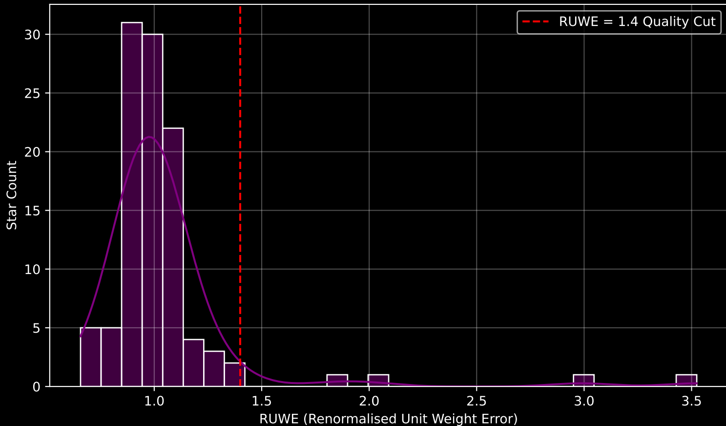
GAPOGEE DR17 Field [005+03] RUWE Distribution (n= 106)
