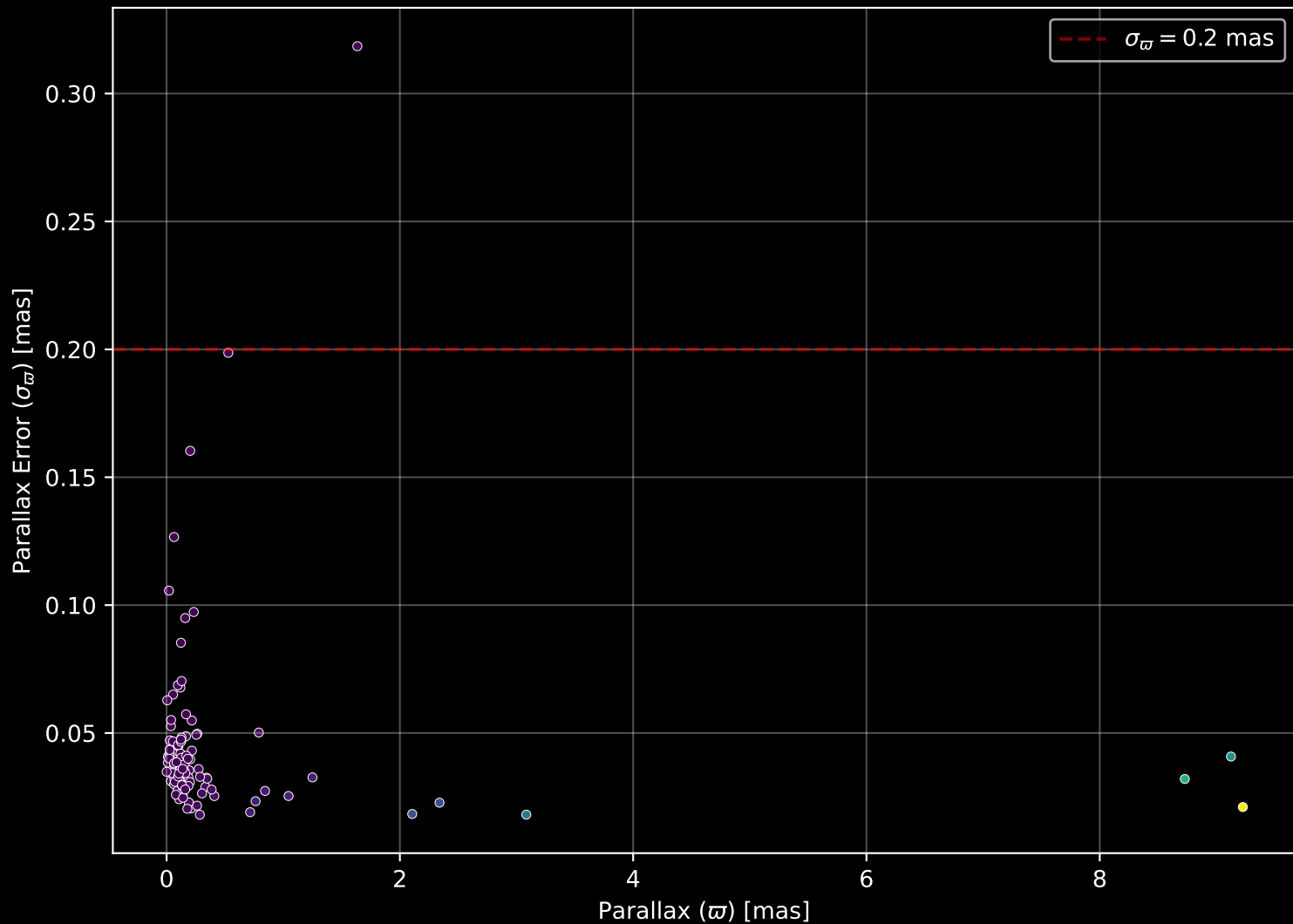
APOGEE DR17 Field: [005+03] Parallax Quality (n= 108)
