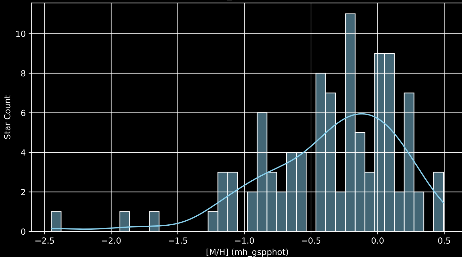
APOGEE DR17 Field: [005+03 [M/H] (mh_gspphot) (n= 99)
