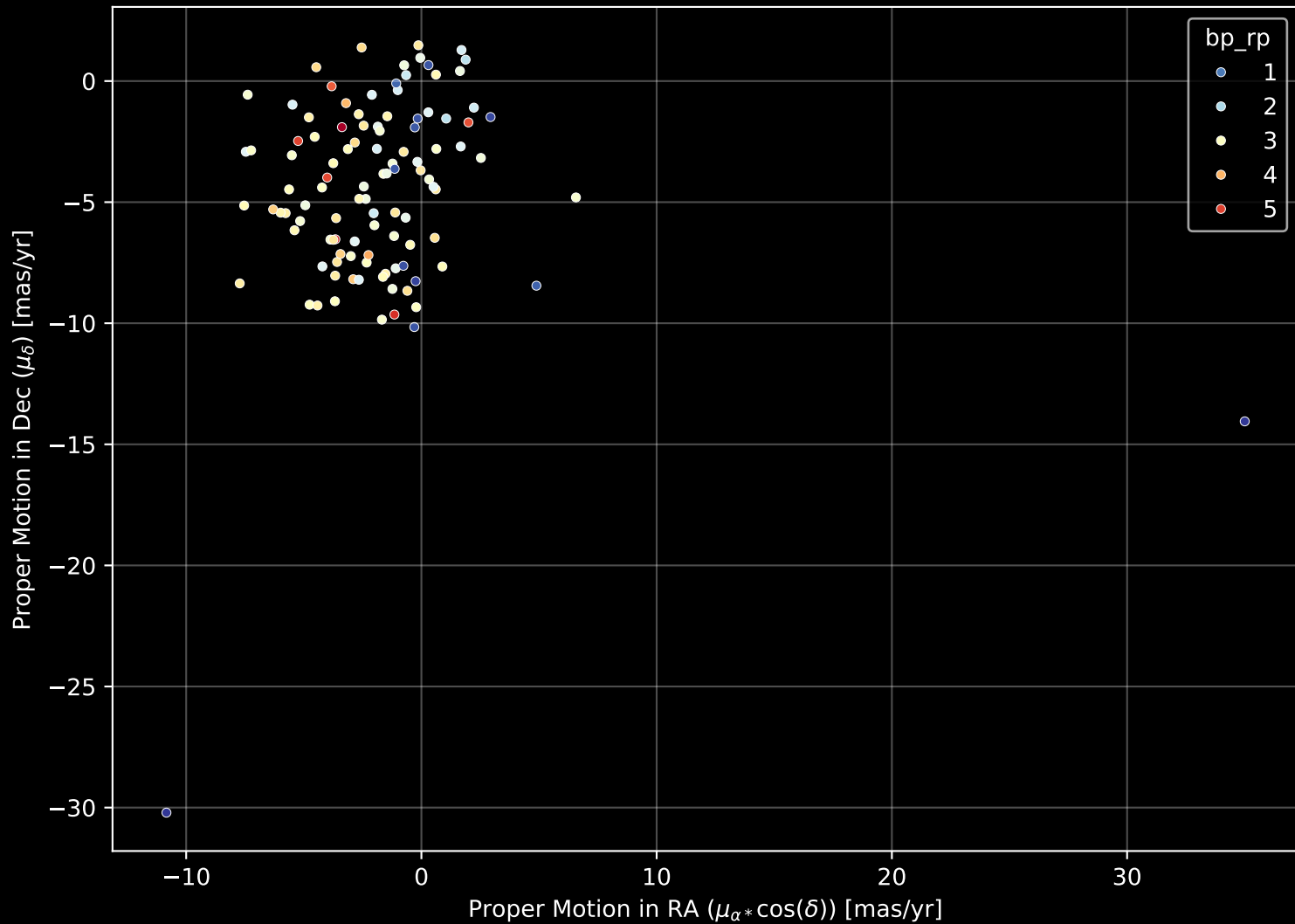
APOGEE DR17 Field: [005+03] Proper Motion Diagram (n= 108)
